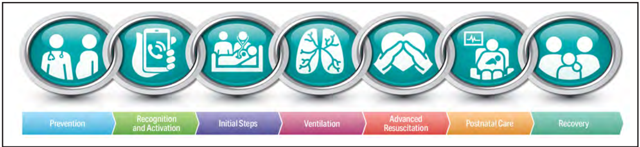
Figure 2. Newborn Chain of Care.
